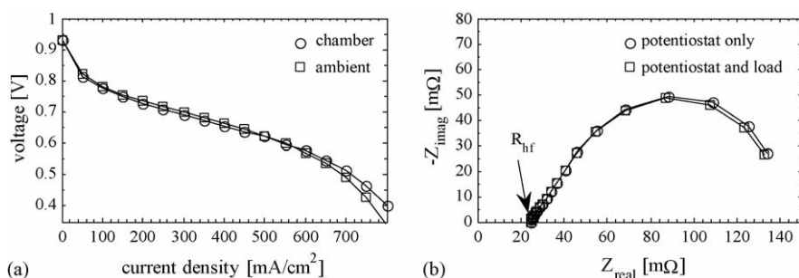
Fig. 4. (a) Overall effect of the environmental chamber on performance of the air-breathing cell under following conditions: 21 °C, 50% RH, Nafion 112 MEA with 1 mg cm -2 Pt loading, 30 s delay between each data point. (b) Effect of the input impedance of the active load on impedance spectra. The EIS measurements were performed with and without the active load. In both instances the fuel cell operating point was 450 mA at 806 mV and the excitation voltage was 10 mV.
