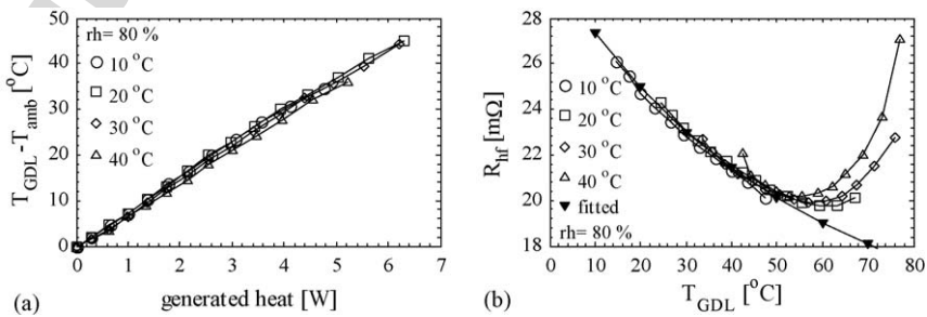
Fig. 12. (a) Temperature difference between GDL surface and ambient as a function of heat generated by the cell at 80% relative humidity and four ambient temperatures and (b) high frequency resistance as a function of GDL surface temperature, at 80% relative humidity and four ambient temperatures. The high frequency resistance is a good measure of membrane resistance and membrane hydration.
