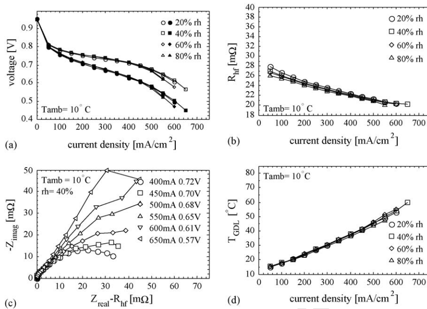
Fig. 10. Measured fuel cell data at 10 °C ambient temperature: (a) polarization (solid) and IR-compensated (open) polarization curves; (b) high frequency resistance as a function of current density; (c) modified impedance plot of fuel cell impedance at 10 °C ambient temperature, 40% ambient relative humidity, and with current density as parameter. The plot legend shows the current density and the IR-compensated fuel cell potential; and (d) GDL temperature as a function of the current density.
