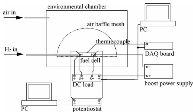
Fig. 3. Schematic of the experimental setup in an environmental chamber. The cell is surrounded by a hemispherical wire mesh shell to diminish the effects of forced convection inside the environmental chamber. Inside the chamber the air temperature and humidity were kept constant at a preset value. We fed cold, dry air into the chamber for improved humidity control and to retain constant partial pressure of oxygen. An active load controlled the operating point of the cell. The cell temperature was monitored by a thermocouple and cell impedance was measured with a potentiostat.
